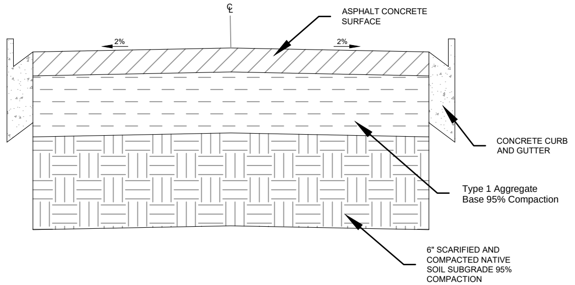
TYPICAL STREET STRUCTURAL CROSS SECTION N.T.S.
